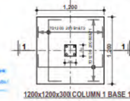
SECTION 1-1
