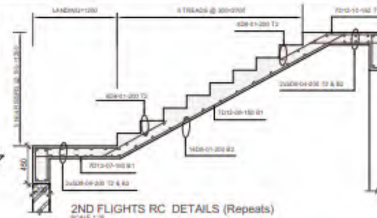
2ND FLIGHT RC DETAILS (Repeats) SCALE 1:25
