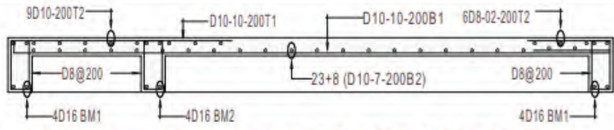
LONGITUDINAL SECTION THRU R.C. SOLID SLAB SCALE 1:25
