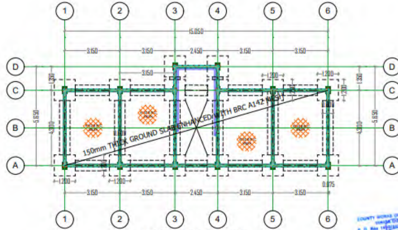
FOUNDATION LAYOUT
