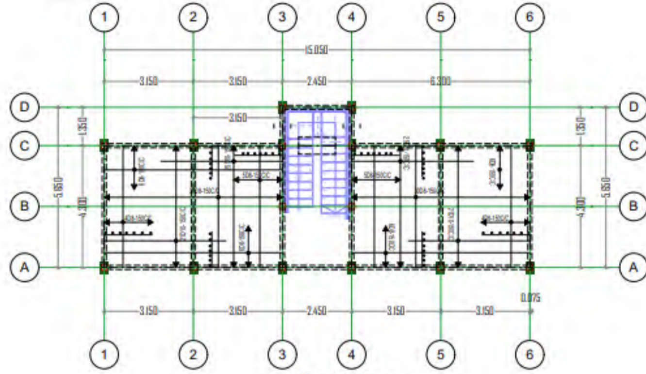
SLAB DETAILS
