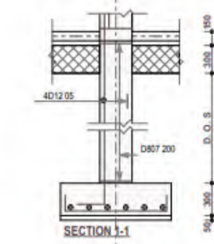
1200x1200x300 COLUMN 3 BASE 3
