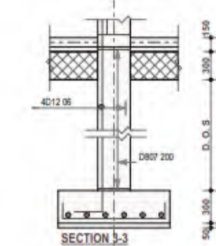
SECTION 3-3
